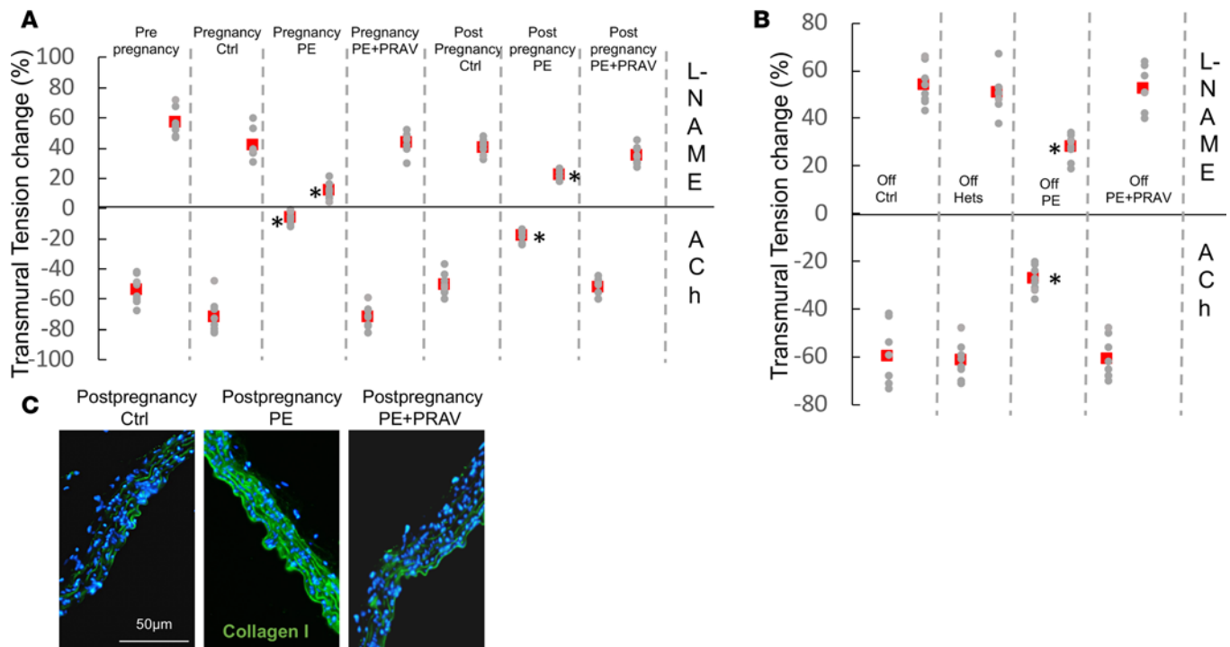
Figure 1. Endothelial function during and after preeclampsia. Wire myography results showing relaxation induced by 3 \mu M acetylcholine (ACh) in precontracted (1 \mu M phenylephrine) endothelium-intact aortic rings from mothers ( A ) (60 days postpartum) after normal pregnancies and pregnancies affected by preeclampsia (PE) treated and untreated with PRAV and the offspring ( B ) (postnatal day 30) ( n = 7-8 mice/experimental group). Effects of NO synthesis inhibitor L-NAME (100 \mu M) are also shown. Red squares represent the mean. The top row in A and B represents the response to L-NAME, and the bottom represents responses to ACh. Comparisons between groups were performed by ANOVA with Bonferroni's post hoc test. * P < 0.05 , different from control, same time point; # P < 0.05 , different from prepregnancy. ( C ) Collagen I deposition in maternal aorta after normal pregnancies and pregnancies affected by PE (untreated and treated with PRAV) ( n = 7-8 mice/experimental group). Increased collagen I deposition (green fluorescence), indicative of fibrosis, is observed in maternal aortas 60 days after PE. Pravastatin given during pregnancy prevented aortic fibrosis. Scale bar: 50 \mu m.
